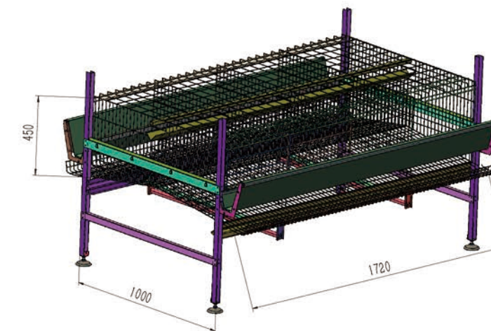
Model 1 3D diagram of egg breeder raising equipment
